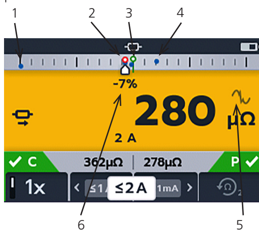
DLRO2 color display with new Difference Meter
