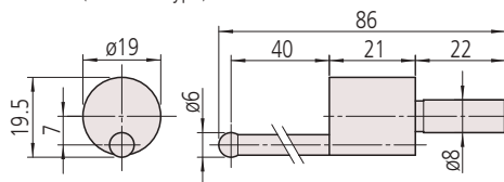
9) 12AAA792 Holder for dial indicator
