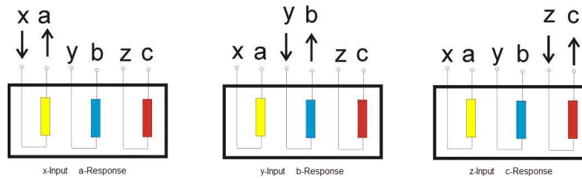
Figure 6 Exterior Connection \Delta Wiring
