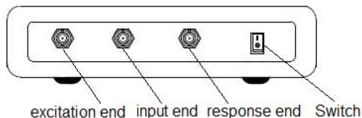
Figure 1a Figure of Transformer Winding Deformation Tester Panel (Front Panel)
